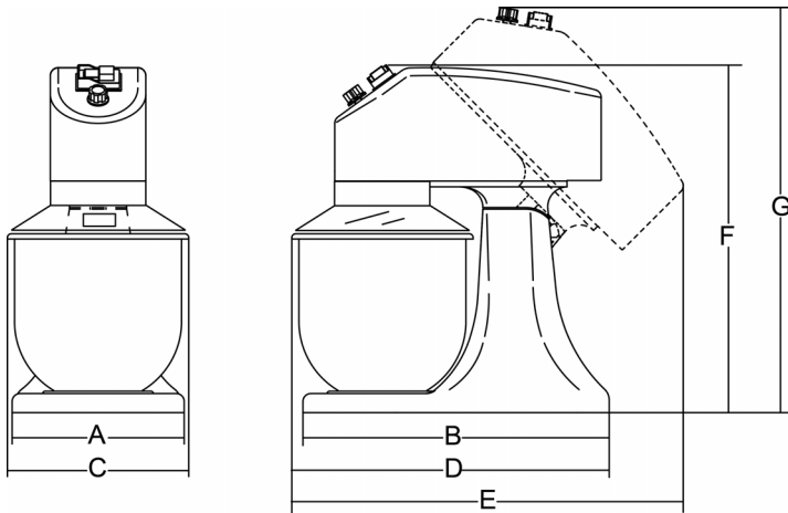
FIG. n.2 - Overall dimensions
