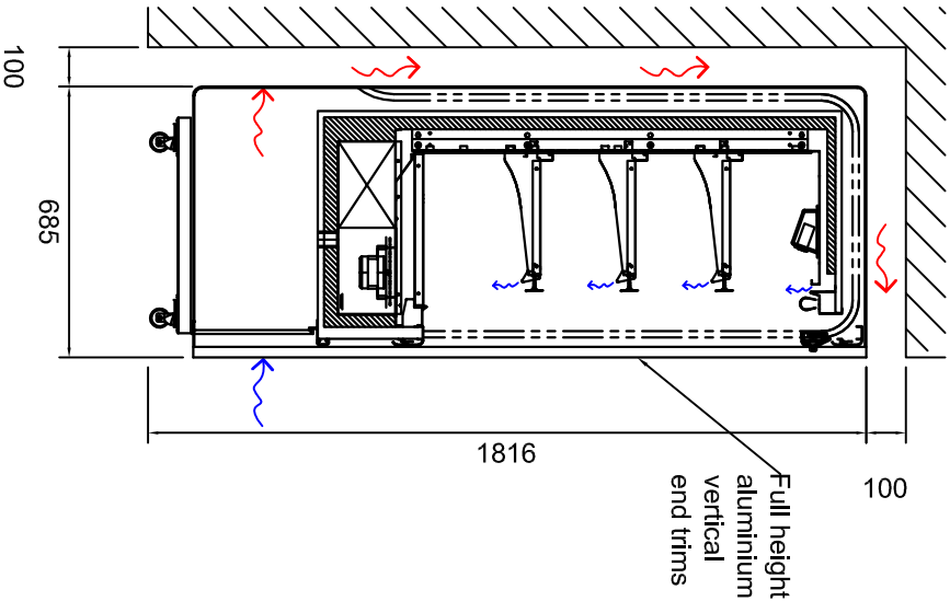
Side Elevation (Ventilation Space)
