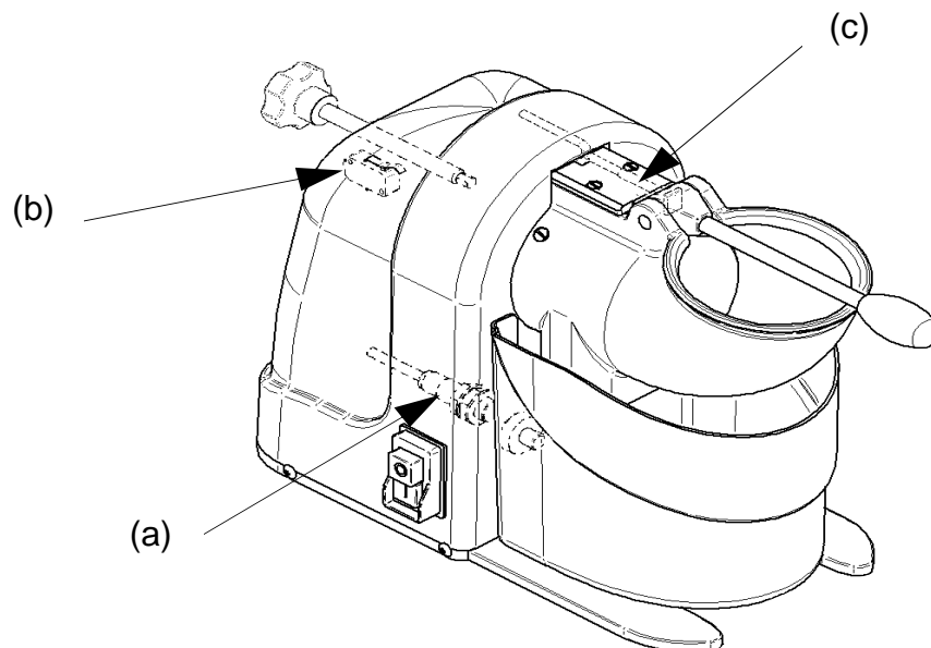
Fig. n°7 - Positions of safety micros
