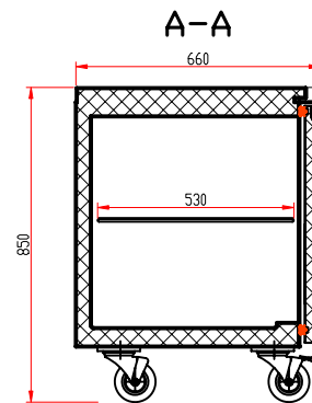
SECTION VIEW
