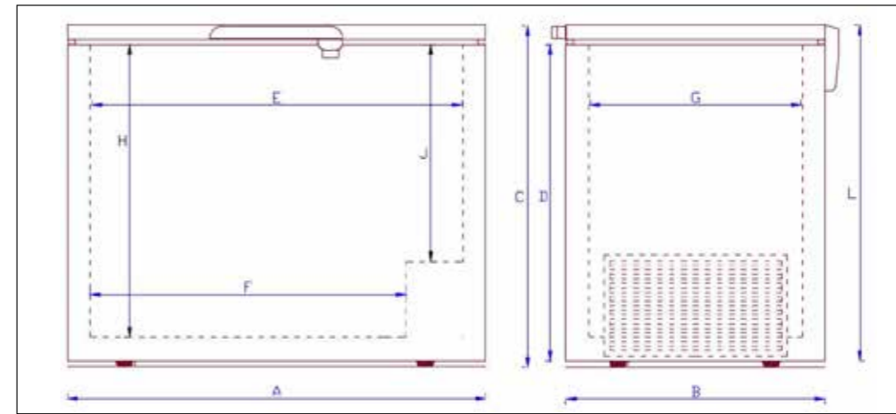
100 MM INSULATION
