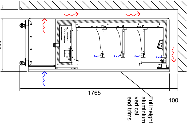
Side Elevation (Ventilation Space)
