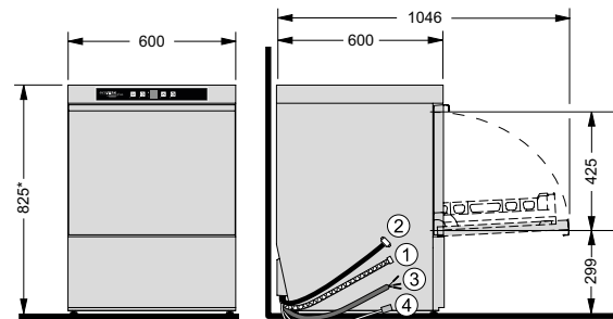
Glasswasher model G515 Undercounter dishwasher model F515
