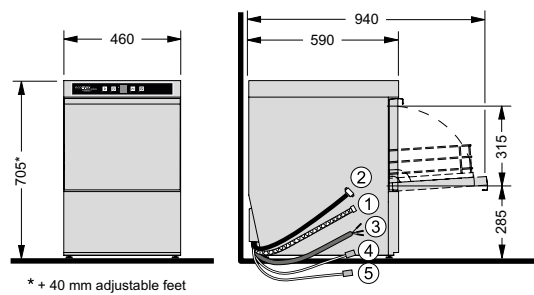
Glasswasher model G415
