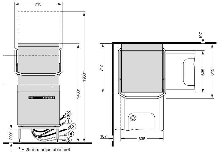
Hood-type dishwasher model H615
