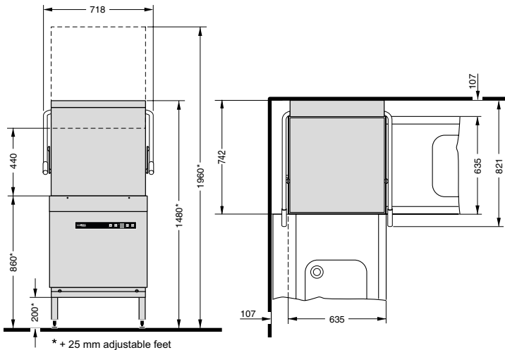
Hood-type dishwasher model H604
