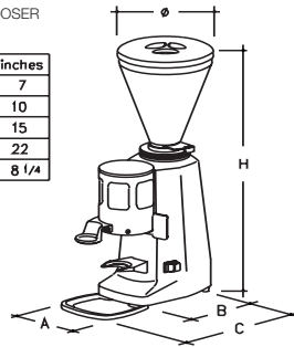
COFFEE GRINDER SUPER JOLLY
