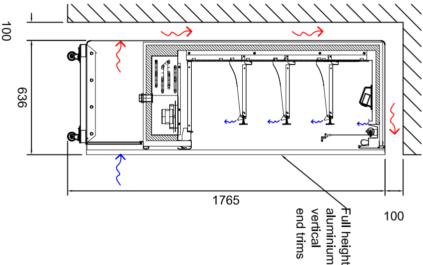
Side Elevation (Ventilation Space)
