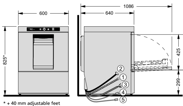
Undercounter dishwasher F515L
