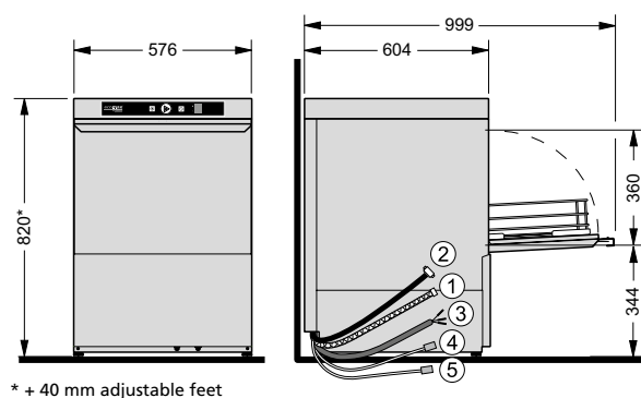
Undercounter dishwasher F504
