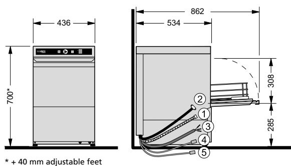
Glasswasher G404
