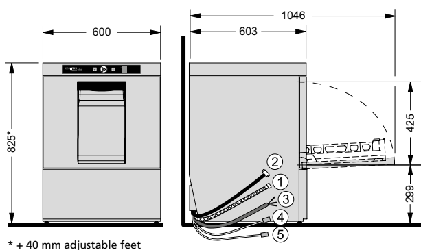
Undercounter dishwasher F515
