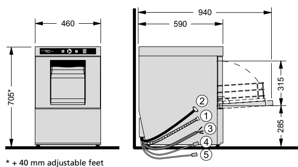
Glasswasher G415
