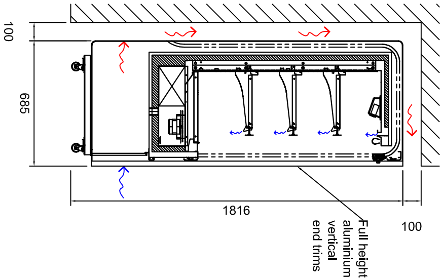
Side Elevation (Ventilation Space)
