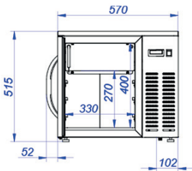
SP0315BC Dimensions
