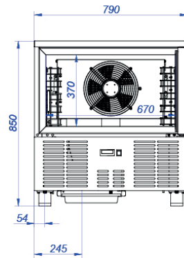
SP0523BC Dimensions
