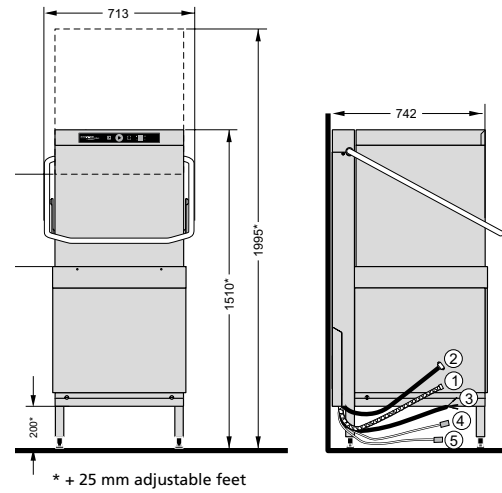
Hood-type dishwasher H615
