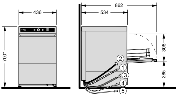
Glasswasher G404
