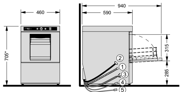
Glasswasher G415
